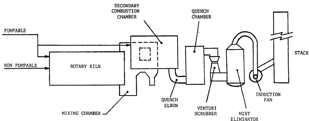
FIGURE 3. Chemolite incinerator schematic.
