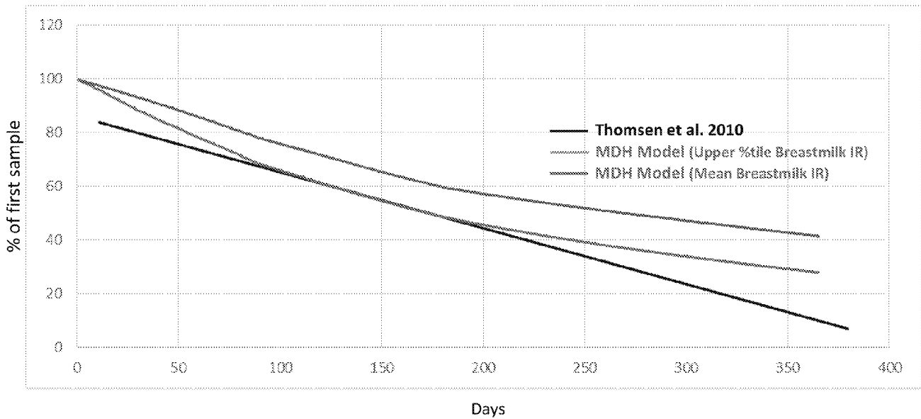
Figure 3. Relative concentration comparison of PFOA in breastmilk*, Thomsen, 2010 and MDH TK model results.
